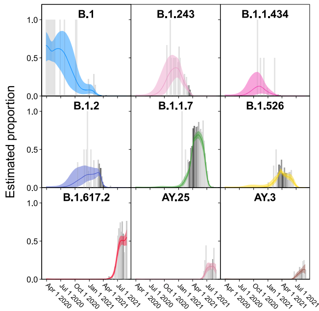
FIG 3 Frequencies of individual variants estimated using Bayesian autoregressive moving average multinomial logistic regression. Time is shown along the x axis and estimated proportions of the surveillance population along the y axis. The gray bars indicate raw proportions from the count data shaded by the number of observations observed in a given week (darker indicating more samples) while the colored lines indicate the proportion estimated by the Bayesian model. The light-colored envelopes around each line show the 95% credible intervals for the proportion. Only lineages achieving an estimated proportion of >10\% in any given week are shown.
